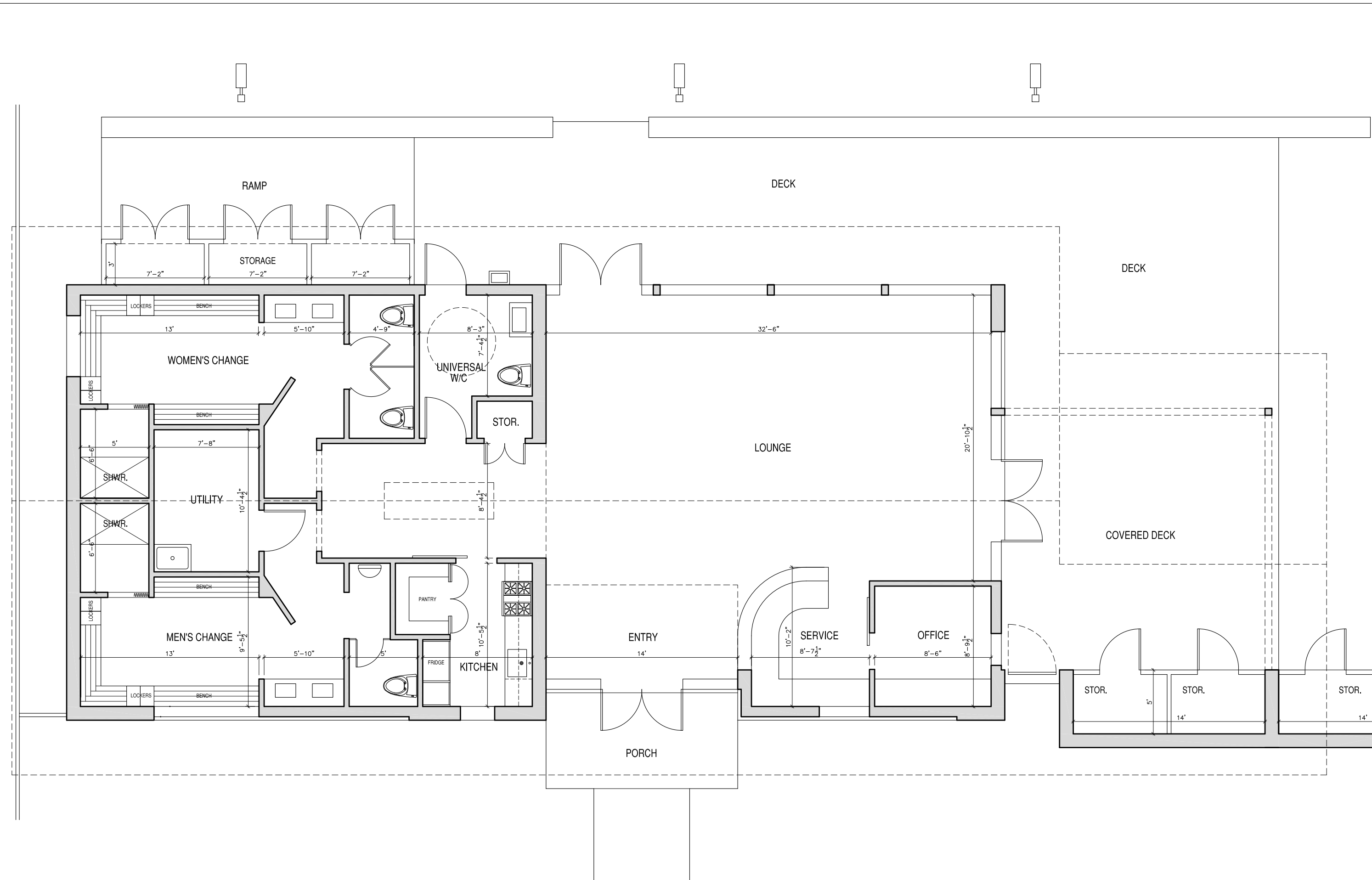
KINGSTON TENNIS CLUB - GROUND FLOOR PLAN
